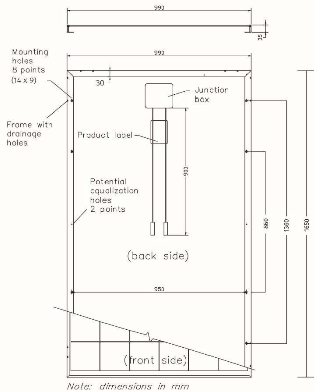
Mechanical drawing 60 cell module
