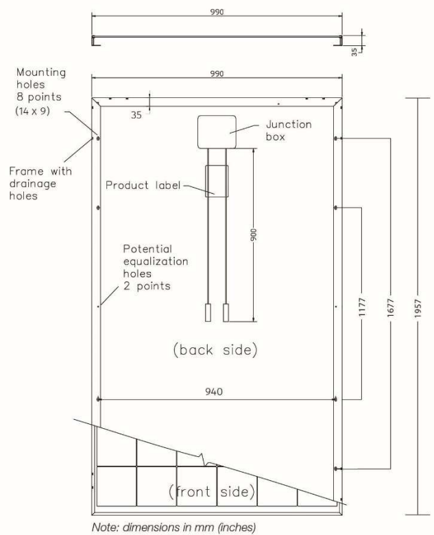
Mechanical drawing 72 cell module
