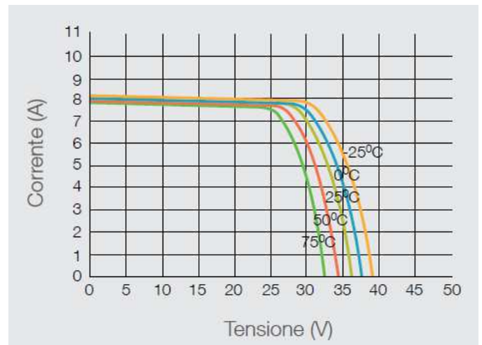
Fig. 1: IV curve at different irradiances
